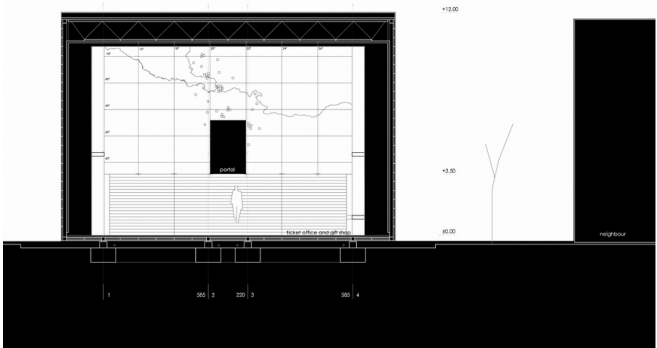
SECTION 2-2 scale 1:100
